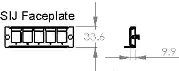
6 Way MPO Adapter Faceplate
